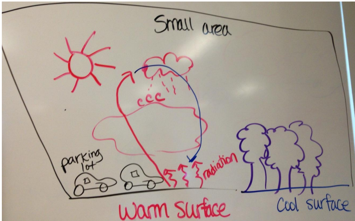
4. Local Convective Lifting
